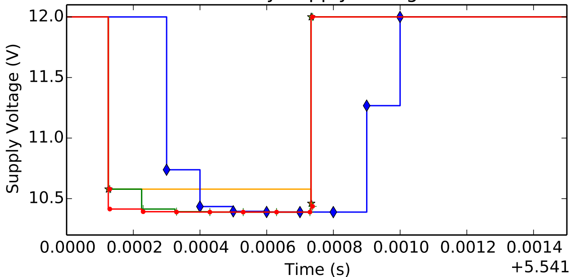
Battery Supply Voltage
