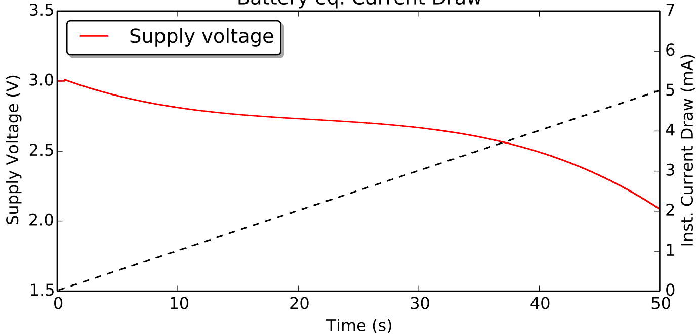
Battery eq. Current Draw
