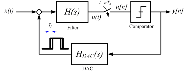
Figure 1: Continuous-Time \Sigma\Delta modulator.
