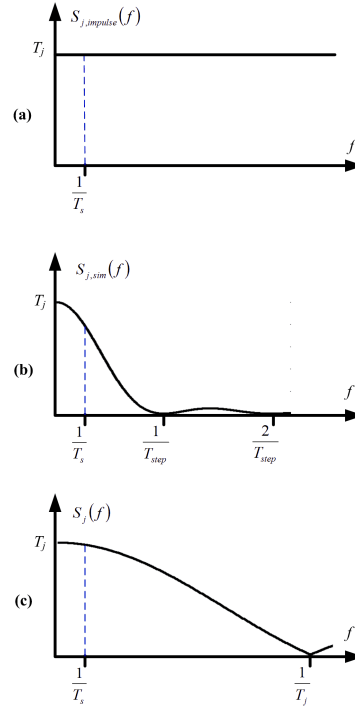
Figure 8: Spectrum of jitter noise. (a) Approximated as impulses [3]. (b) Proposed model. (c) Exact model.
