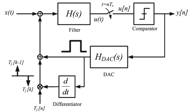
Figure 5: Proposed jitter simulation model.
